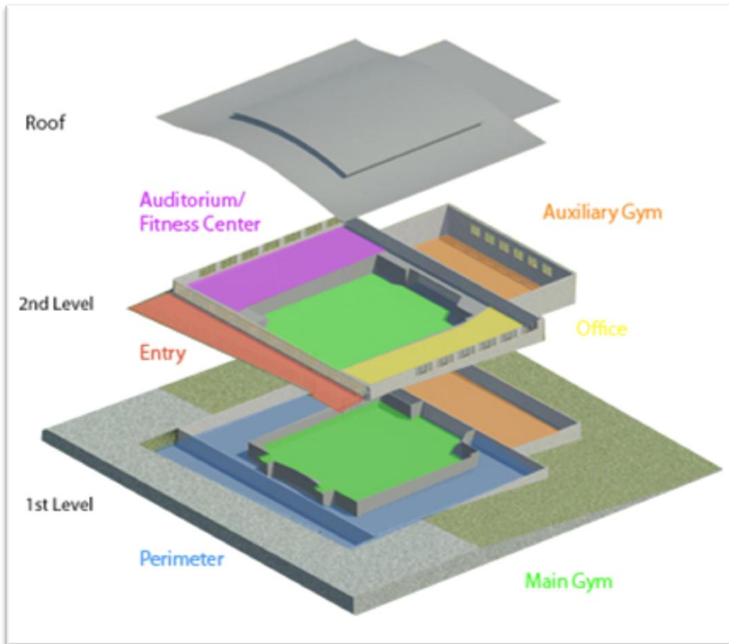
Exploded View
